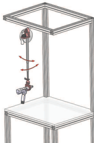
DMF AAPC Equipped with two angle encoders (inclinometer)
