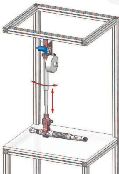
DMF LAPC Equipped with one length encoder and one angle encoder
